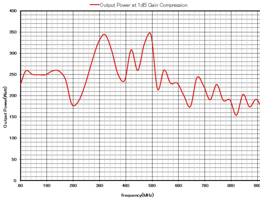
Model ZSA5252-80M1G Typical Power Output
